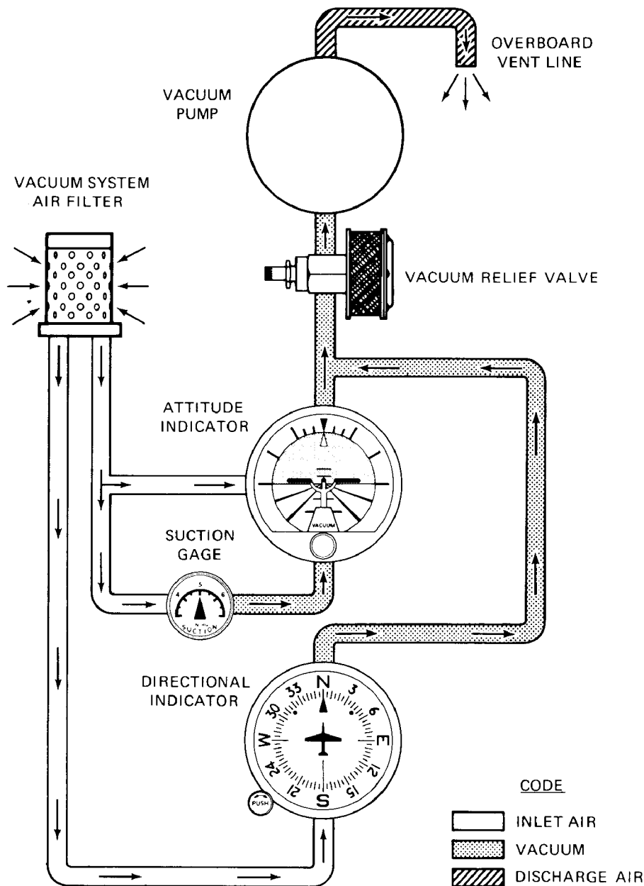
Figure 7-9. Vacuum System
