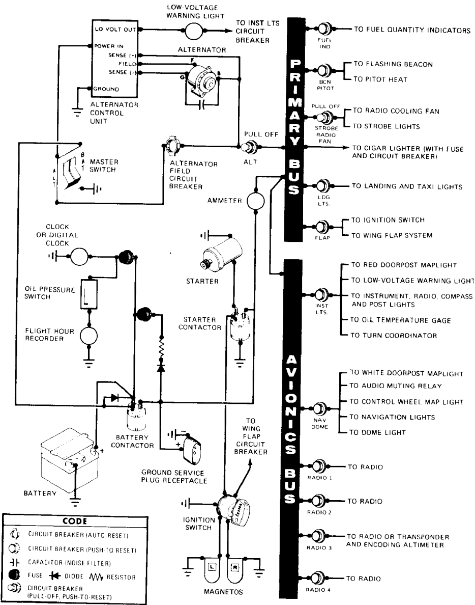
Figure 7-7. Electrical System
